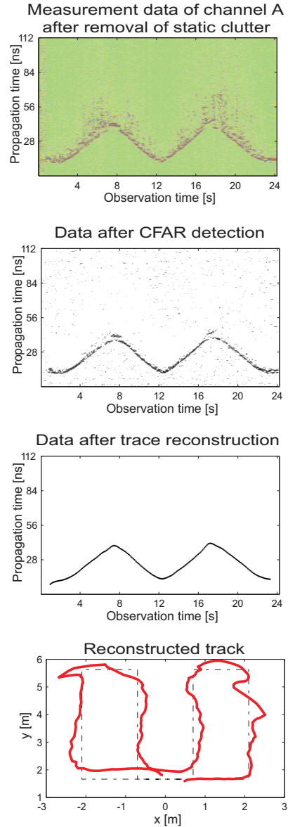
Fig. 5. Data processing steps for moving people tracking
