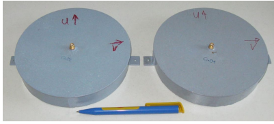
Fig. 3. Spiral antennas for through-wall imaging
