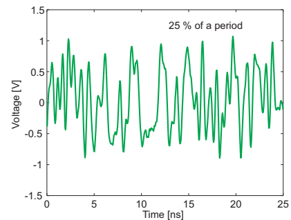
Fig. 1. Time shape of the emitted wave form
