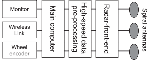
Fig. 4. Schematics of the trough wall imaging radar
