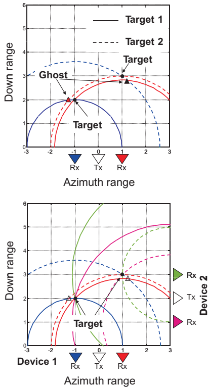
Fig. 6. Creation of ghost targets by a simple 3-element antenna array (above) and their suppression by second radar (below)
