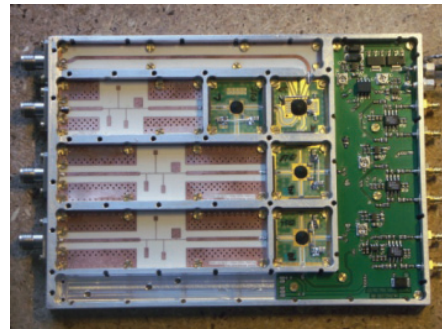
Fig. 2. RF-front end consisting of one transmitter and two receiver channels
