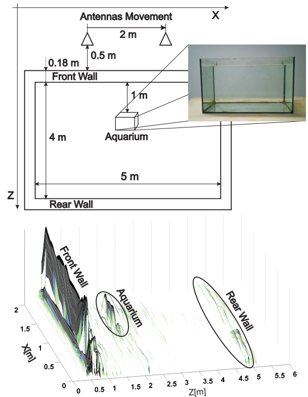
Fig. 8. SAR experiment resulting in correct target positions after respecting wave propagation in the wall
